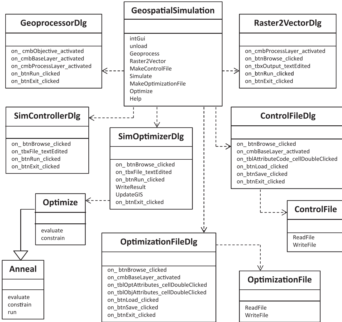
Fig. 2. A class diagram for the Geospatial Simulation (GeoSim) plug-in. The methods for each class are given, but the attributes are excluded for simplicity.
