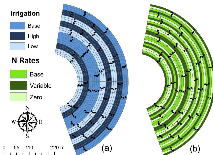
Fig. 5. Experimental design for a 14 ha agronomic study near the city of Lamesa in west Texas, where site-specific seed cotton yield was tested in response to a) variable irrigation management and b) variable nitrogen fertilizer management. Soil texture variability was characterized from soil samples at 135 sampling points (black circles) across the study area.
