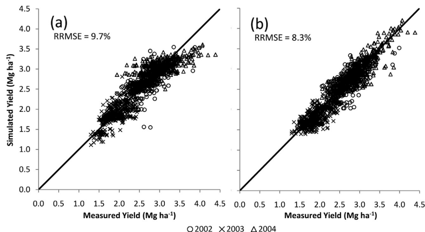
Fig. 8. Simulated versus measured spatial seed cotton yield for three growing seasons after spatially optimizing the drained upper limit soil parameter for the a) AquaCrop model and b) the DSSAT Cropping System Model.
