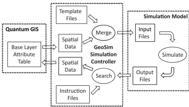
Fig. 4. The Simulation Controller tool within Geospatial Simulation (GeoSim) uses template files to interface the geospatial data from the base layer polygon shapefile with the simulation model input files. It uses instruction files to search model output files for the geospatial data to be returned to the base layer.
