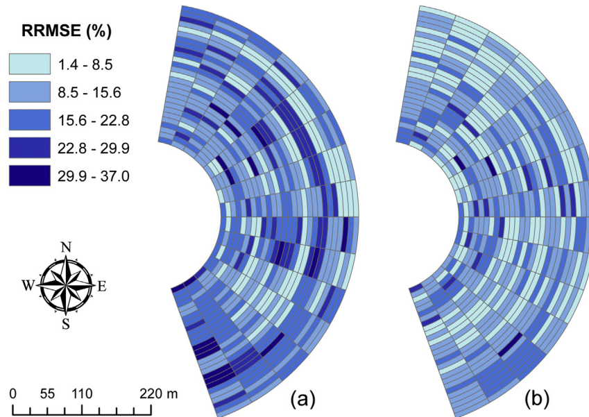
Fig. 7. Spatial distribution of relative root mean squared error (RRMSE) between simulated and measured seed cotton yield for three growing seasons using the a) AquaCrop model and b) the DSSAT Cropping System Model.
