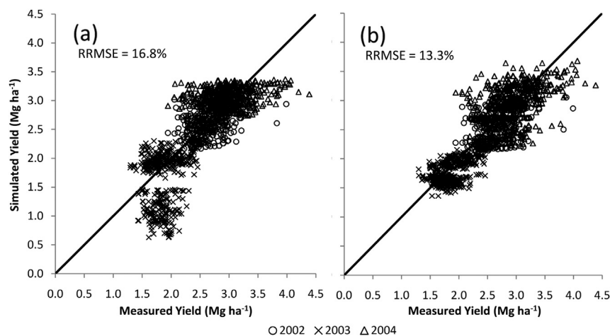
Fig. 6. Simulated versus measured seed cotton yield for three growing seasons using the a) AquaCrop model and b) the DSSAT Cropping System Model.
